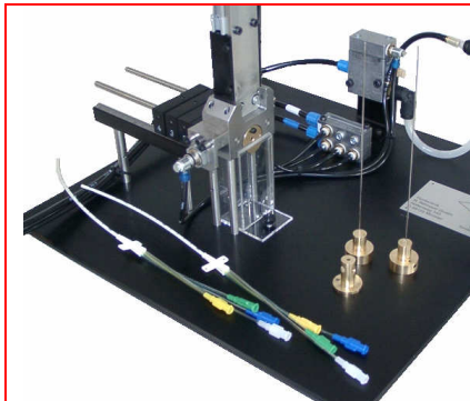
Catheter cutting machine for four miscellaneous lumen tubes in different diameters.
